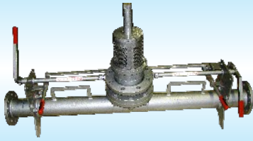
Rail Tanker T Pipe Discharge Valve For Petrol, Diesel and Hazardous Chemicals
