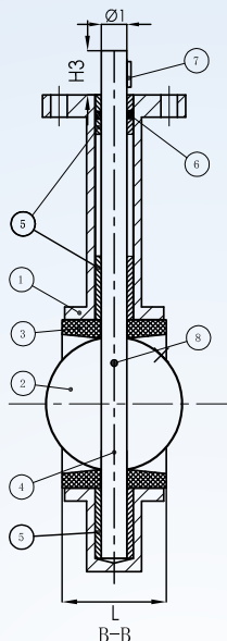
FIG 7777IV BMC CAST IRON WAFER TYPE BUTTERFLY VALVES VITON LINER
