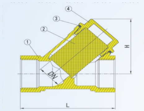
28I STRAINER BRASS
