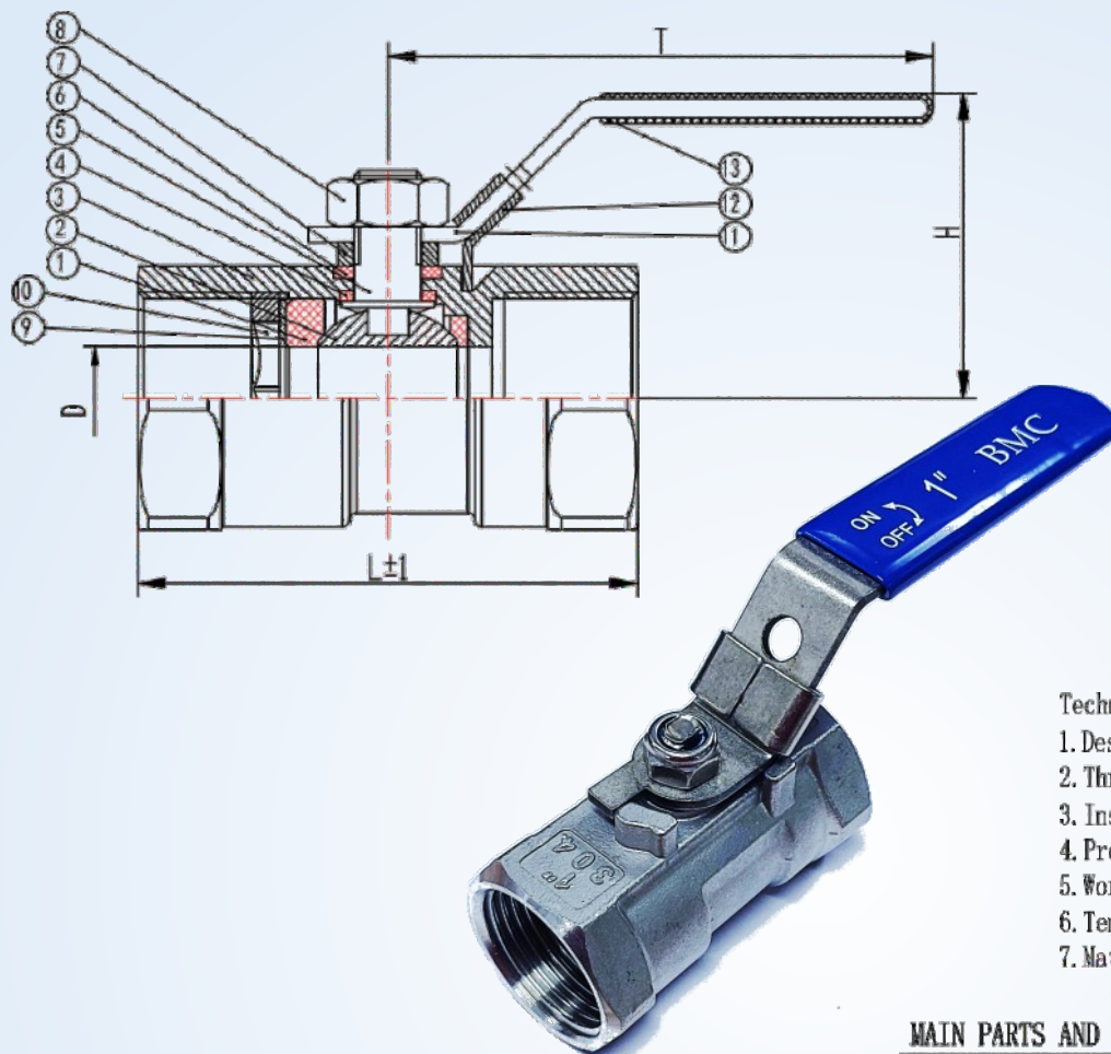
FIG 4164I BMC Ball Valve 1 Piece Reduced Bore 304SS
