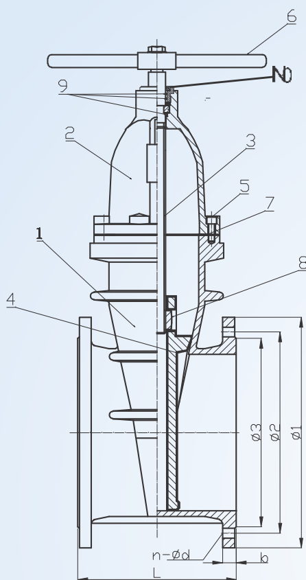
FIG :RSV664 BMC RSV GATE VALVES NON RISING SPINDLE
