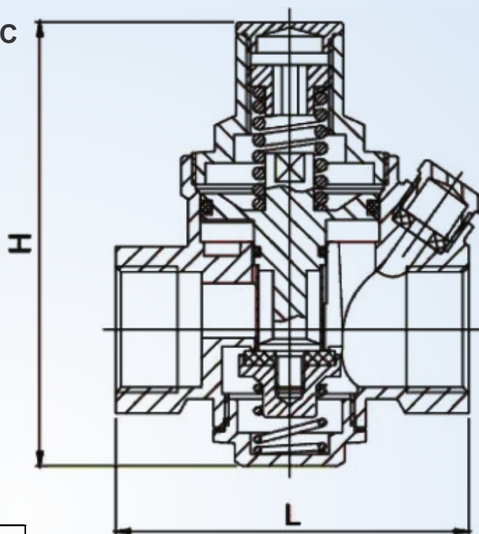
FIG 197I BMC BRASS PRESSURE REDUCING VALVE
