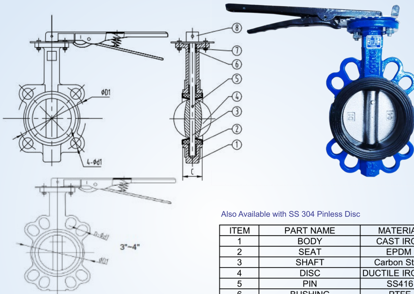
FIG 7777INP C/I WAFER BUTTERFLY VALVE NP & SS DISC
