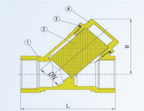
28I STRAINER BRASS
