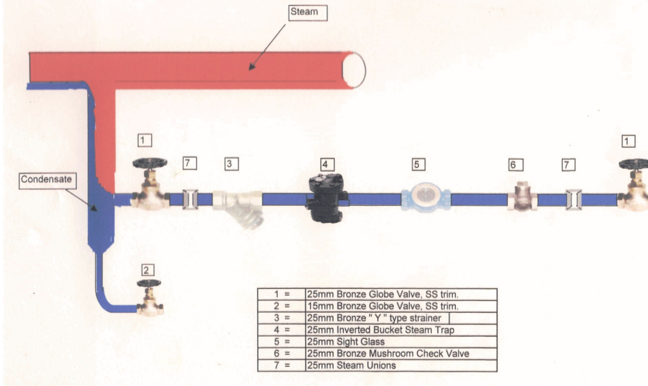
STEAM TRAP SET - INVERTED BUCKET STEAM TRAP
