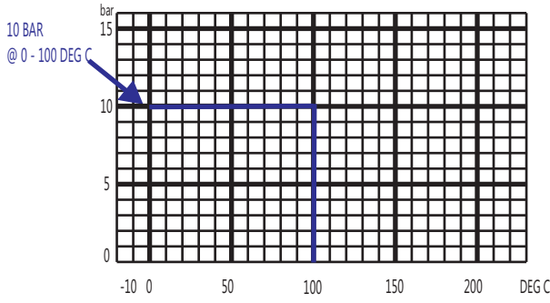
PRESSURE/TEMPERATURE RATINGS
